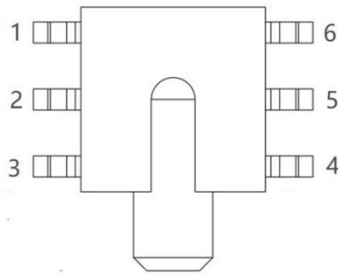
Fig.1 Pin Definition
