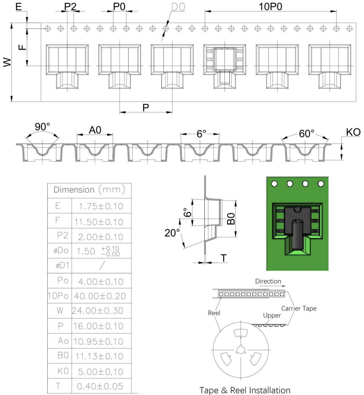
Fig.7 Carrier tape drawings
