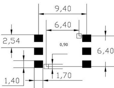
Fig.4 Recommended footprint
