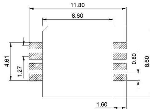
Fig.9 Recommended footprint
