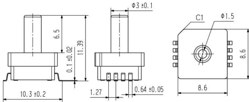
Fig.8 Product dimensions
