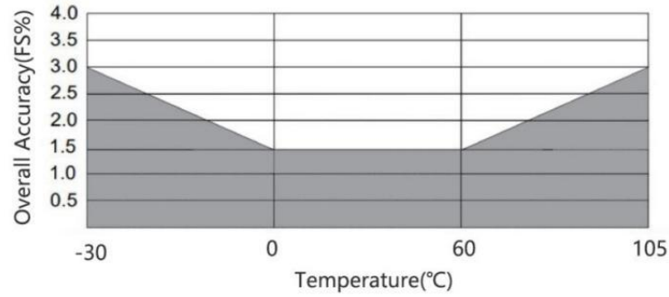
Fig.3 Overall Accuracy vs. temperature.
