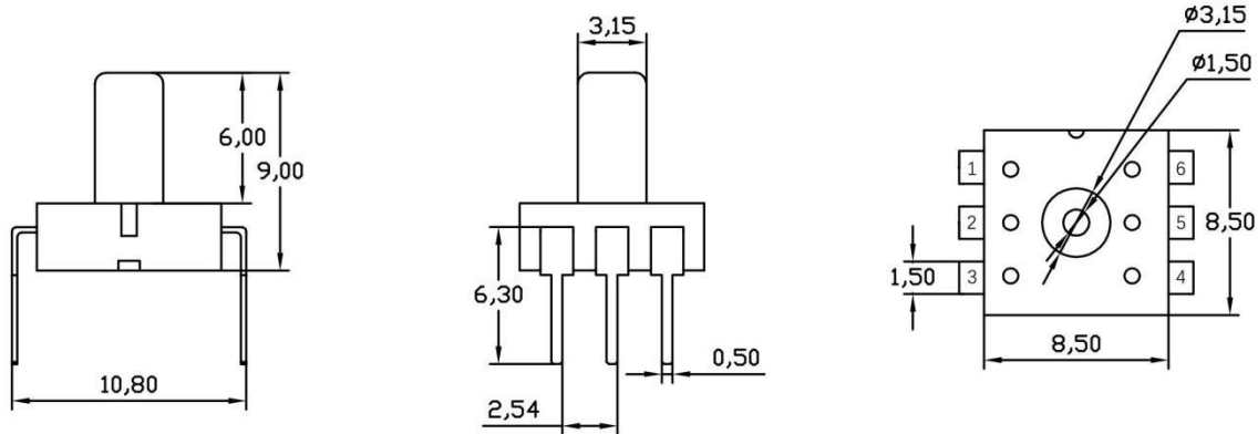
Fig.8 Product dimensions
