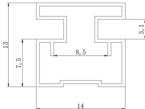
Fig.8 Section schematic diagram
