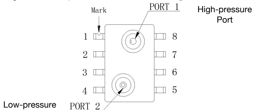
Fig.2 Pin configuration diagram
