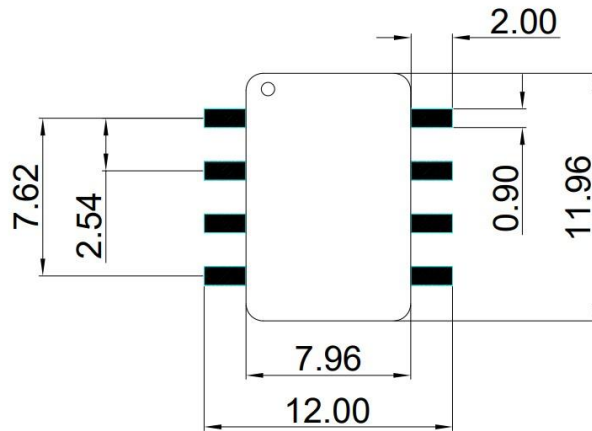
Fig.7 Recommended Footprint
