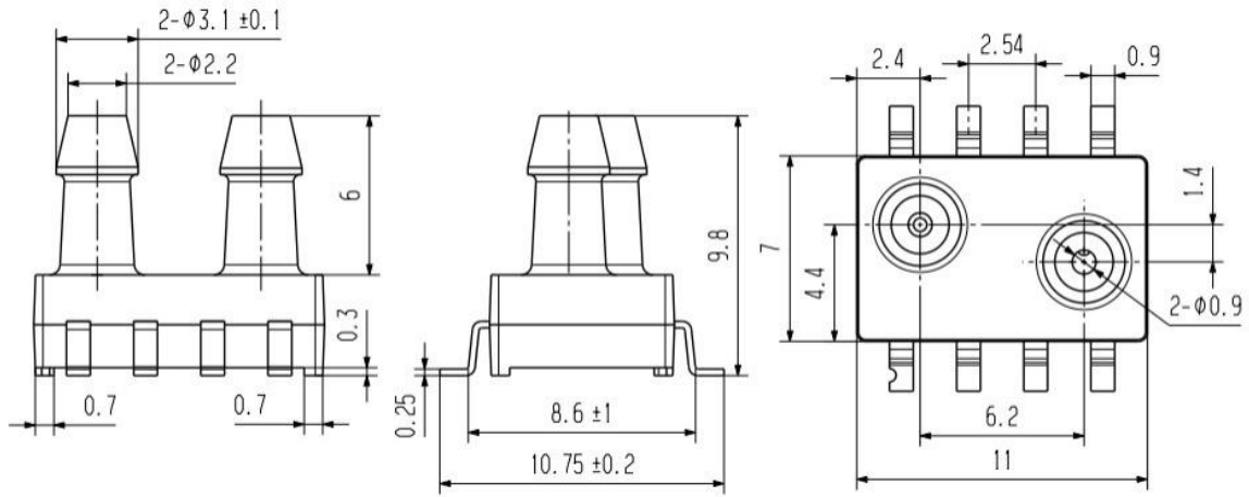
Fig.6 Sensor Dimensions
