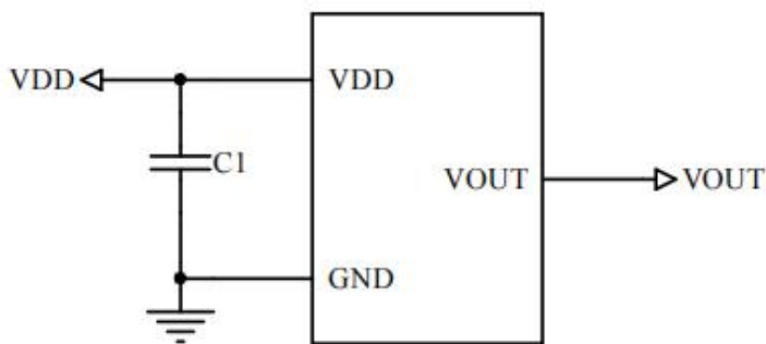
Fig.5 Application circuit
