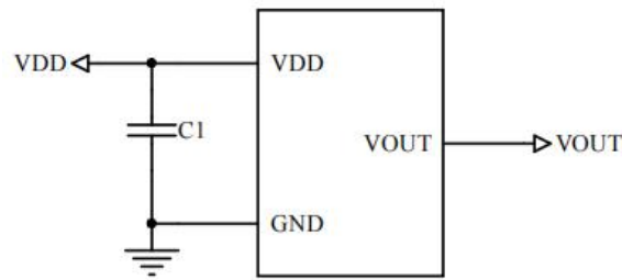
Fig.5 Application circuit
