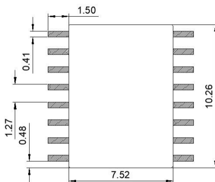
Fig.7 Recommended Footprint
