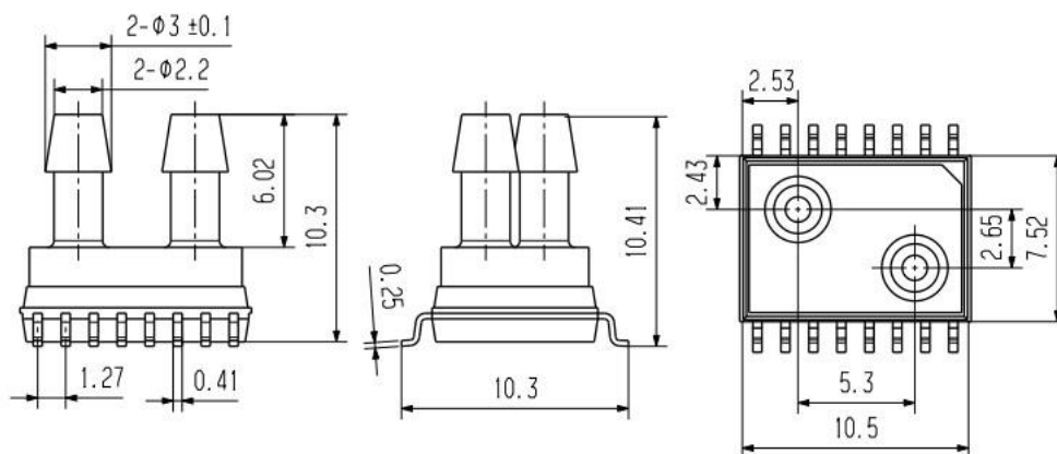
Fig.6 Sensor Dimensions
