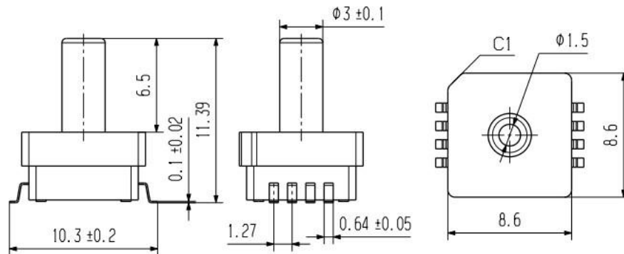
Fig.6 Sensor Dimensions
