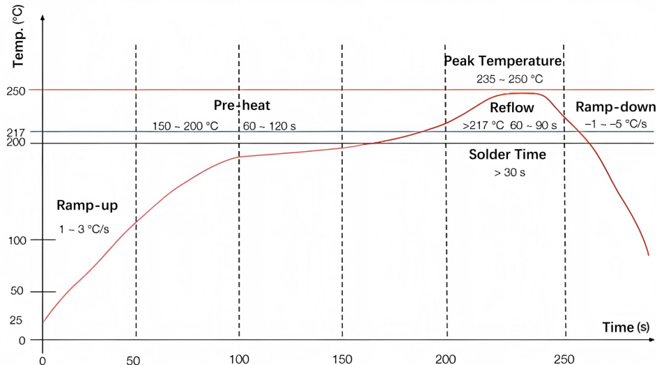
Fig.8 Remelting temperature setting conditions
