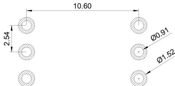
Fig.7 Recommended Footprint
