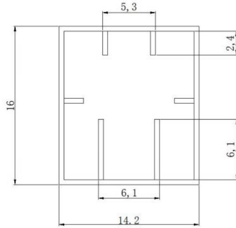
Fig.8 Section schematic diagram
