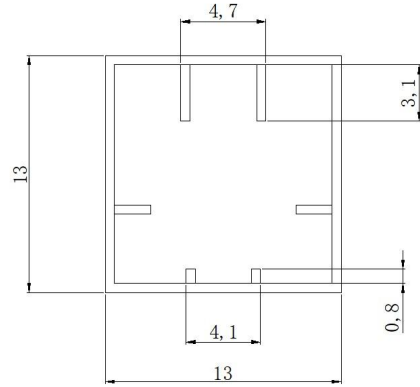
Fig.8 Section schematic diagram
