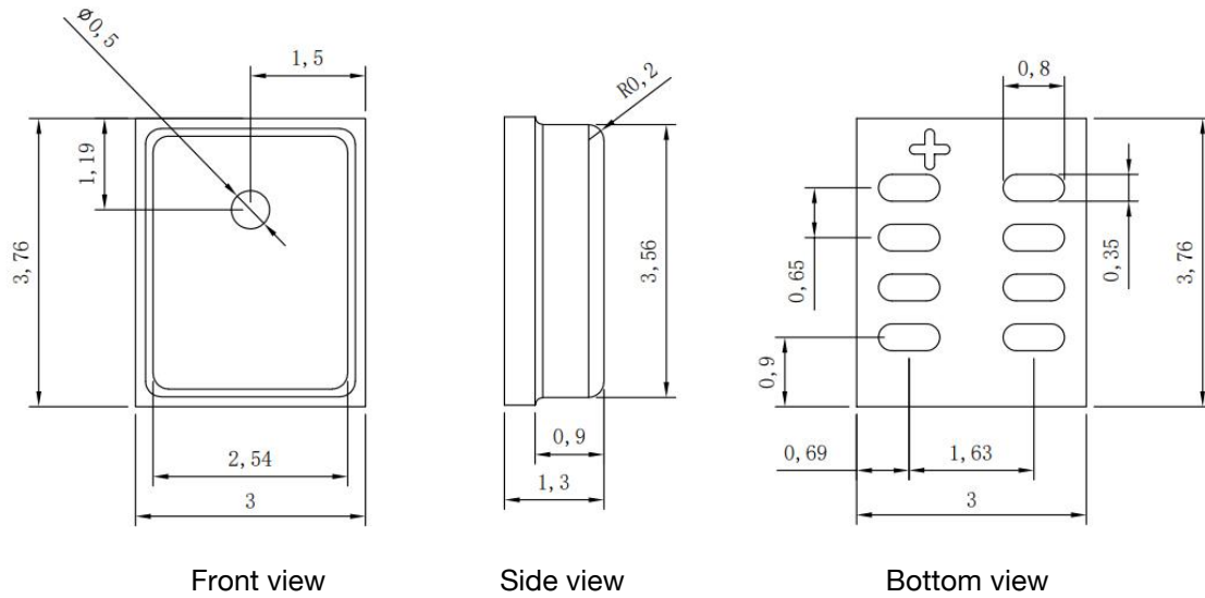
Fig.6 Sensor Dimensions
