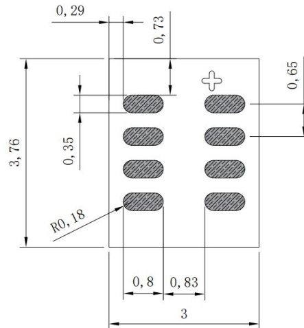
Fig.7 Recommended Footprint
