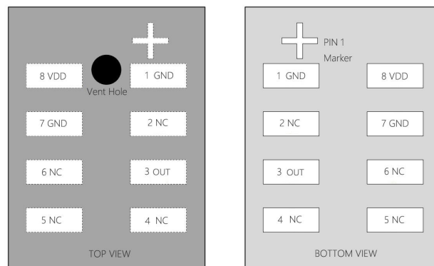
Fig.2 Pin Diagram
